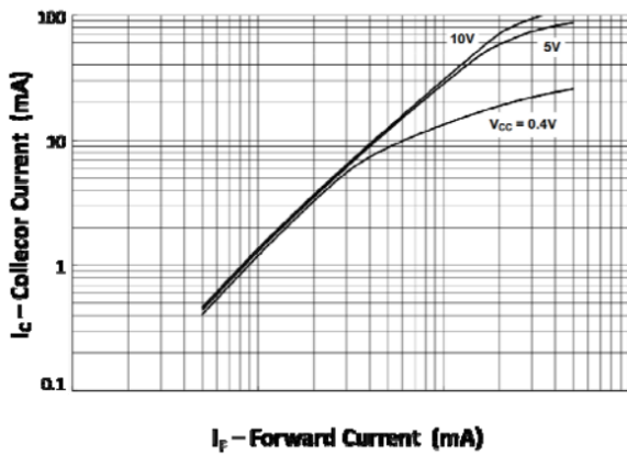
Fig 9 Collector Current vs Forward Current
