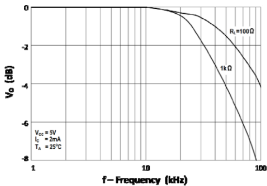
Fig 17 Frequency Response
